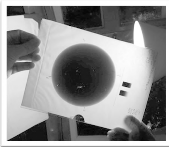
Figure 9: 'Data' in astrophysics. Photo Source: own photo
